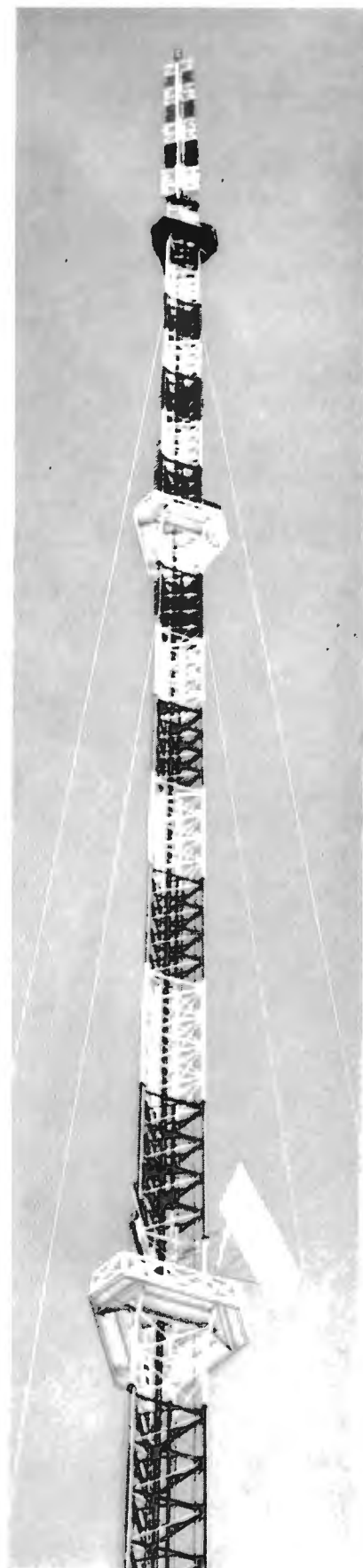
FIG. 2. WKZO, Kalamazoo, Michigan. 40# wind load.
