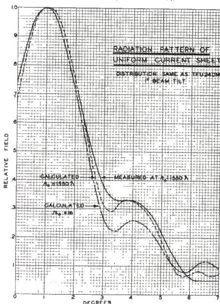
FIG. 15. Radiation pattern of uniform current sheet ( 1^\circ beam tilt).
